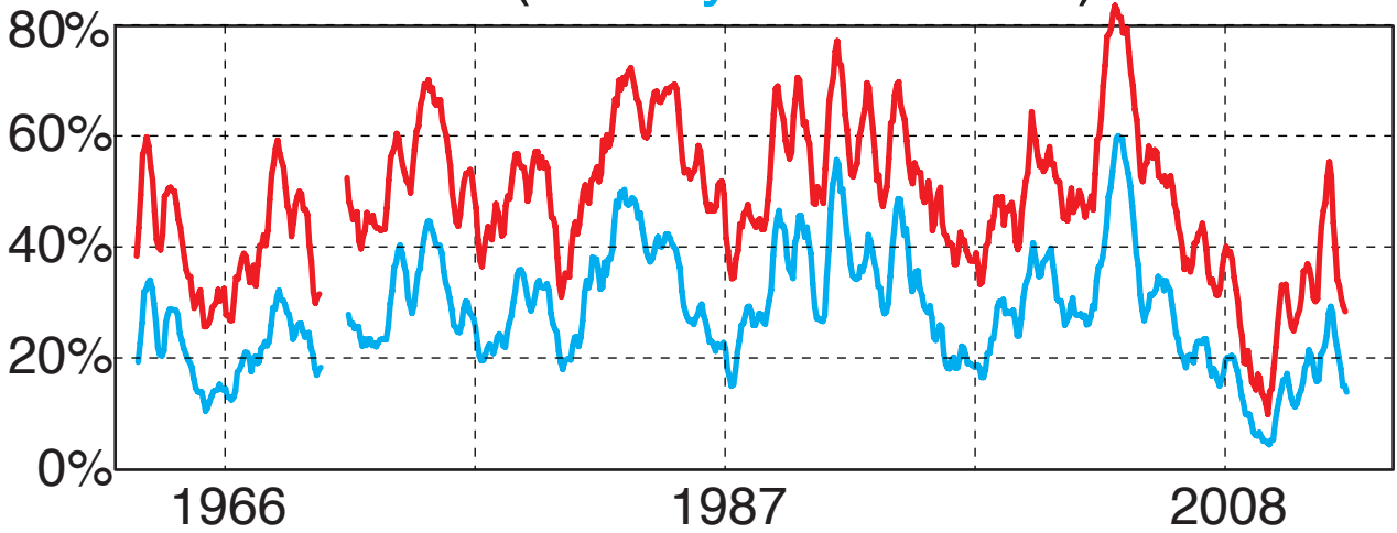
Chance of K \geq 4 (all day / 22-01 LT) @Kiruna
