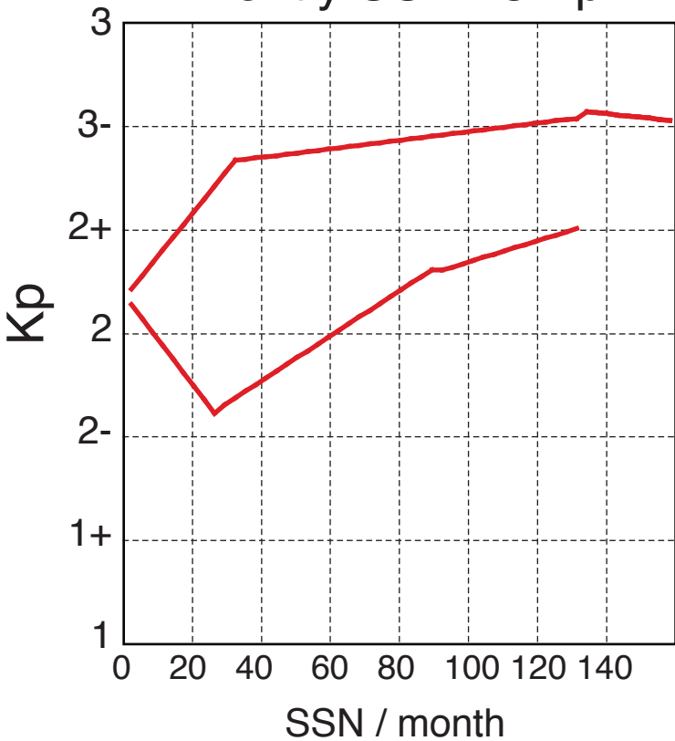
monthly SSN vs Kp
